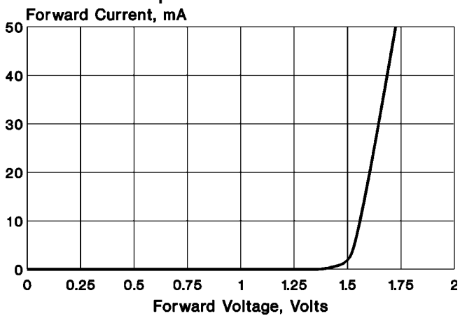
Input Characteristics
