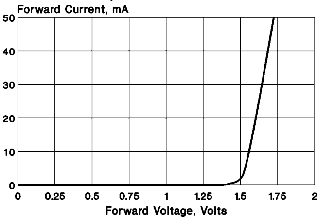
Input Characteristics
