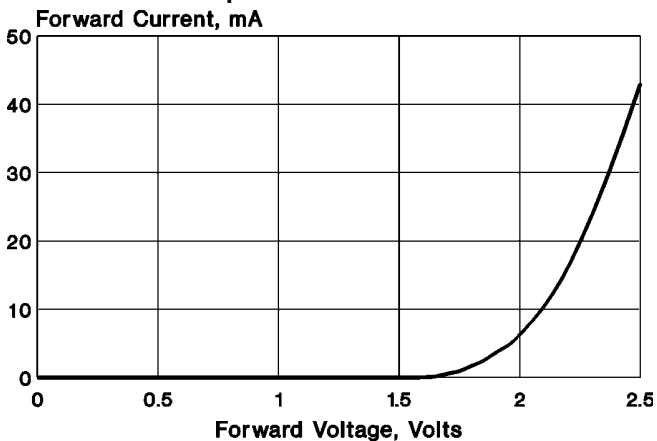
Input Characteristics
